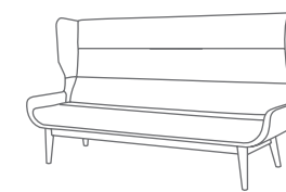
03 HUSH-SF-2000 Hush three seat sofa with timber base metric (mm) W2000 D815 H1160 seat 430 imperial (in) W79 D32 H45.5 seat 17
